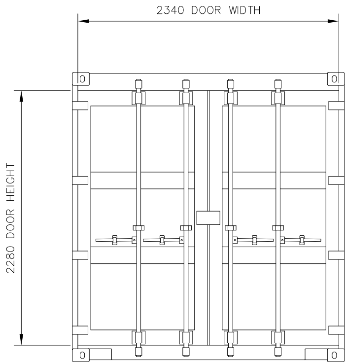
END ELEVATION ON ARROW 'A'
